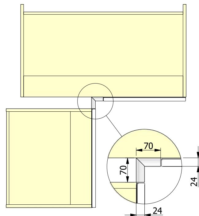
BASE - Type B cpost
