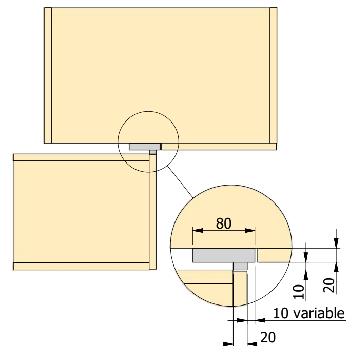
WALL - Type C cpost
