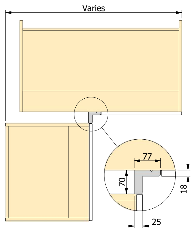
BASE - Type A cpost
