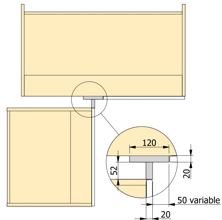
BASE - Type C cpost
