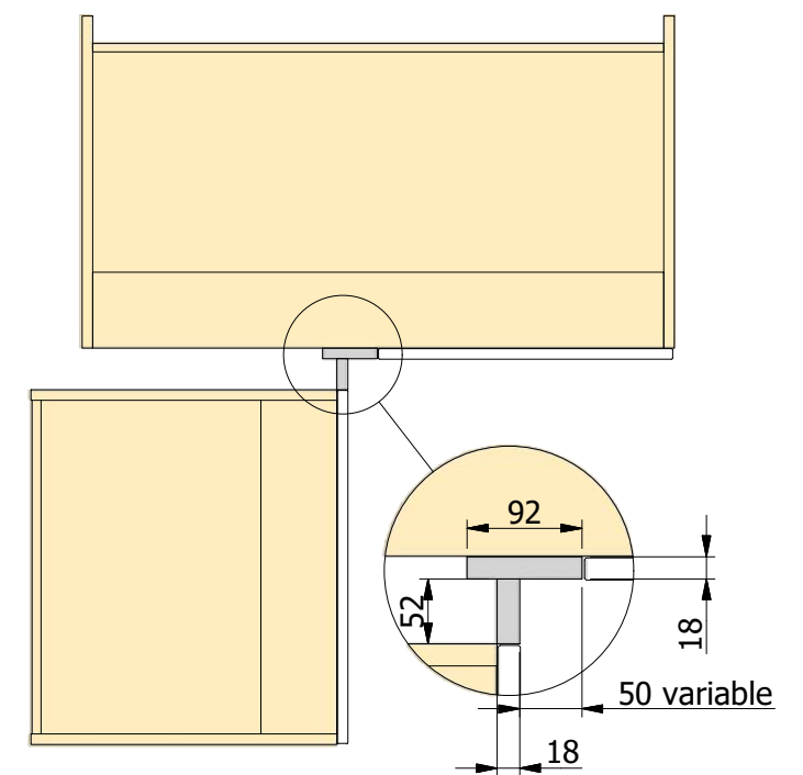
BASE - Type D cpost
