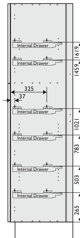
Type 3* Hinged Doors 6 Internal Drawers
