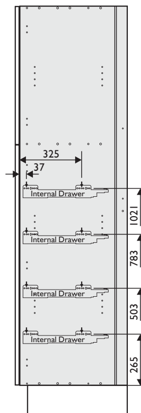
Type 4* Hinged Doors 4 Internal Drawers
