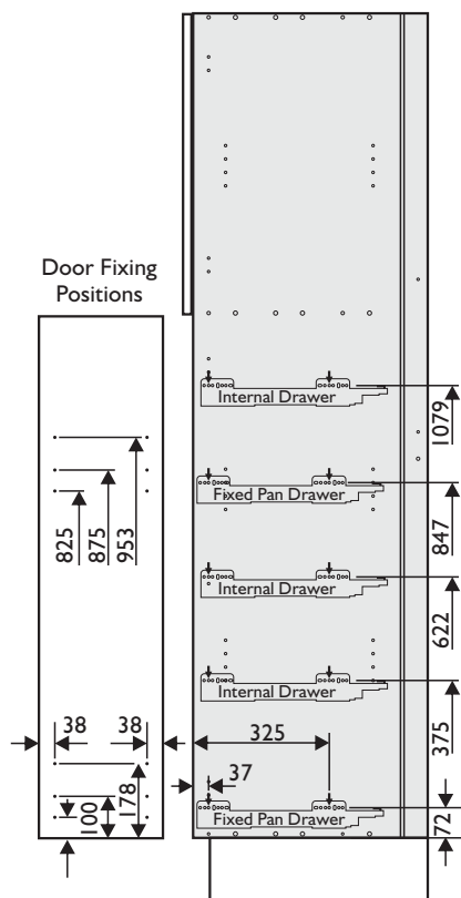
Type 2 Hinged Top Door 3 Internal Drawers 2 Fixed Pan Drawers
