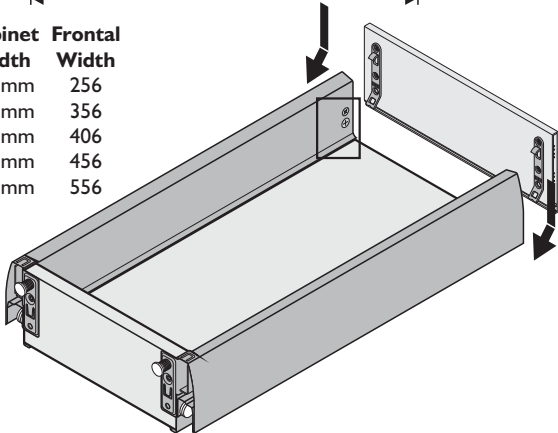
Type 1 1 Working Top Drawer 1 Internal Drawer 1 Fixed Pan Drawer
