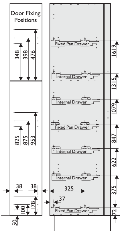
Type 1 4 Internal Drawers 3 Fixed Pan Drawers
