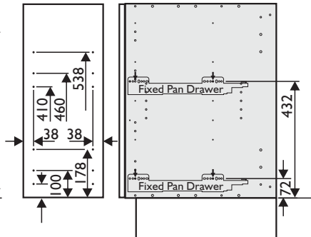
Type 2 Hinged Top Door 3 Internal Drawers 2 Fixed Pan Drawers
